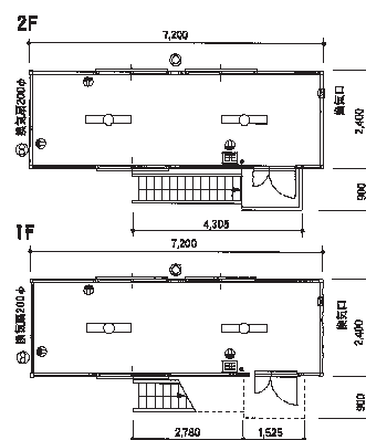
SH-H6 2階建
